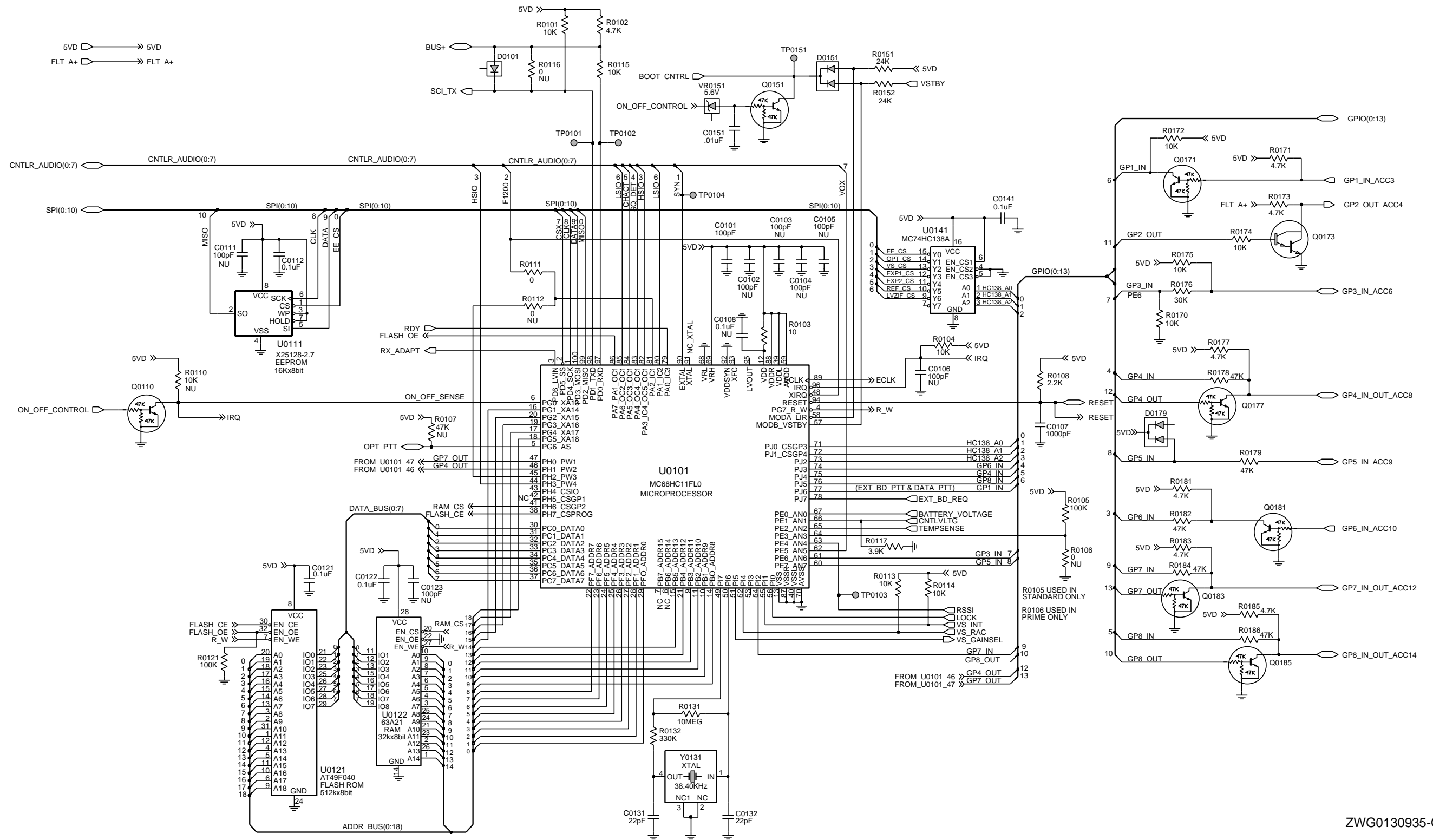
Controller T11 Schematic Diagram - Microprocessor
